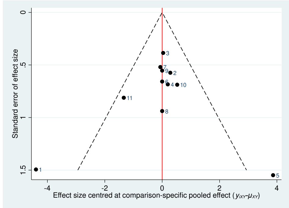
6b-Comparison-adjusted funnel plot for the primary safety outcome (complications) from the network meta-analysis
