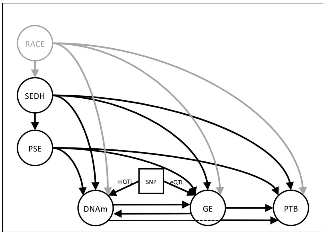
Figure 1 This model illustrates the relationships between environmental factors (left) and how each may affect biological processes (bottom) important to the timing of birth either directly (eg, PSE \rightarrow DNAm ) or indirectly ( PSE \rightarrow DNAm \rightarrow GE ). Chronic stressors are represented by SEDH. Many of those factors are correlated with race and will influence the type of environment a woman experiences during pregnancy. Single headed arrows represent possible causal pathways based on empirical evidence that links SEDH to poor birth outcomes. This framework allows for tests of mediation via DNAm and GE and of moderation effects of DNA sequence (eQTLs/mQTLs). DNAm, DNA methylation; GE, gene expression; PSE, pregnancy-specific environment; PTB, preterm birth; SEDH, social and environmental determinants of health; SNP, single nucleotide polymorphism moderating DNA methylation (mQTL) or GE (eQTL).
