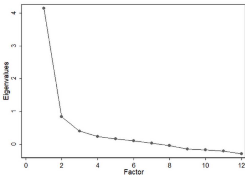
Figure 1 Scree plot for women Note: The graph shows one factors before the inflection point in the curve (eigenvalue >1)
