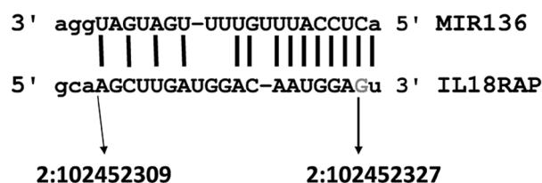
Figure 2 Characteristics of the interaction between MIR136 and IL18RAP . MicroRNA targets predicted using the microRNA.org tool are shown; the base in grey corresponds to the position of the rs7559479 polymorphism.
