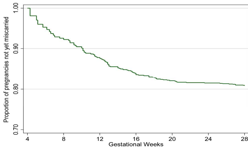
Miscarriage Kaplan Meier survival curve by gestational week. 190x107mm (300 x 300 DPI)
