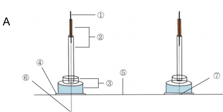
① Needle handle; ②Transparent guide tube; ③Opaque plastic base; ④Double-side tape; ⑤Skin; ⑥Sharp tip; ⑦Blunt tip
